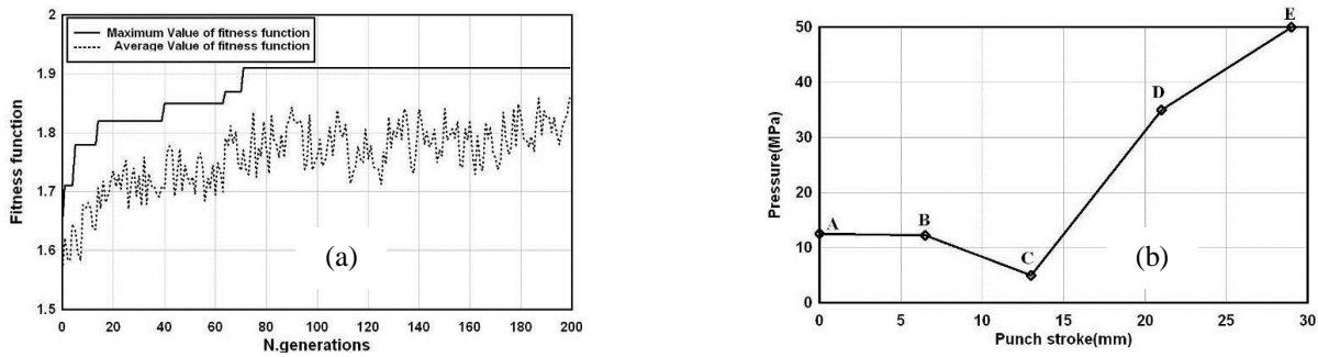
Fig 6. (a) Value of Fitness Function, (b) Optimum pressure path obtained by genetic algorithm
