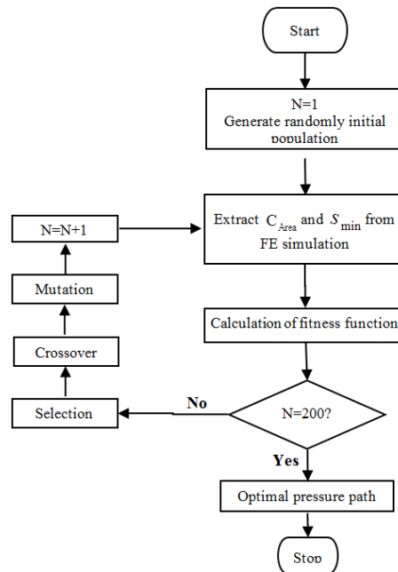
Fig. 4. Flow chart of the optimization procedure
