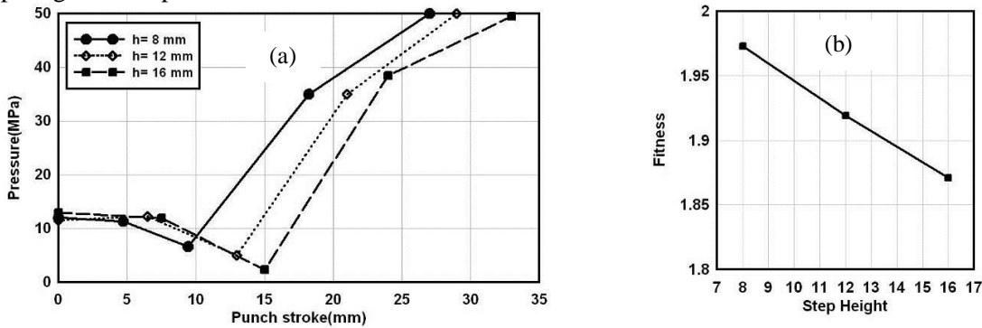
Fig. 9 (a) Optimized pressure curves obtained from genetic algorithm at different step heights of the punch, (b) Variations of the fitness function versus step height
