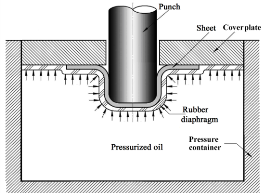
Fig 1. Hydroforming deep drawing process (HDD) [5]
