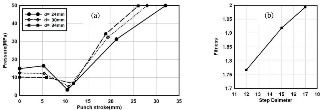
Fig. 10 a) Optimization curve result by genetic algorithm in different diameter of the punch, b) Variations of fitness function with respect to step diameter
