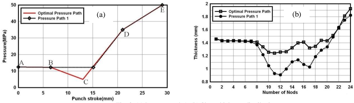
Fig. 8. (a) Pressure path 1, (b) Sheet thickness distribution
