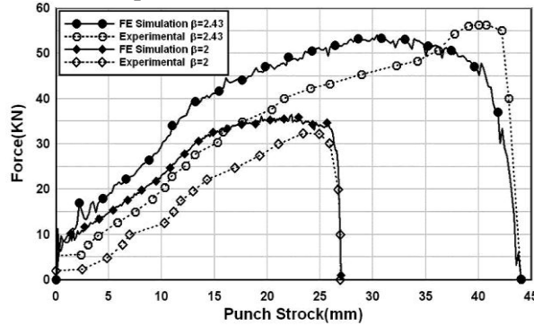
Fig 5. Force- punch stroke curves obtained from simulation and those of experiments of ref. [5]
