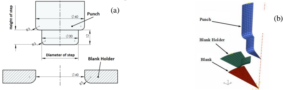
Fig. 2. (a) Dimensions of the punch and blank holder, (b) Finite element model
