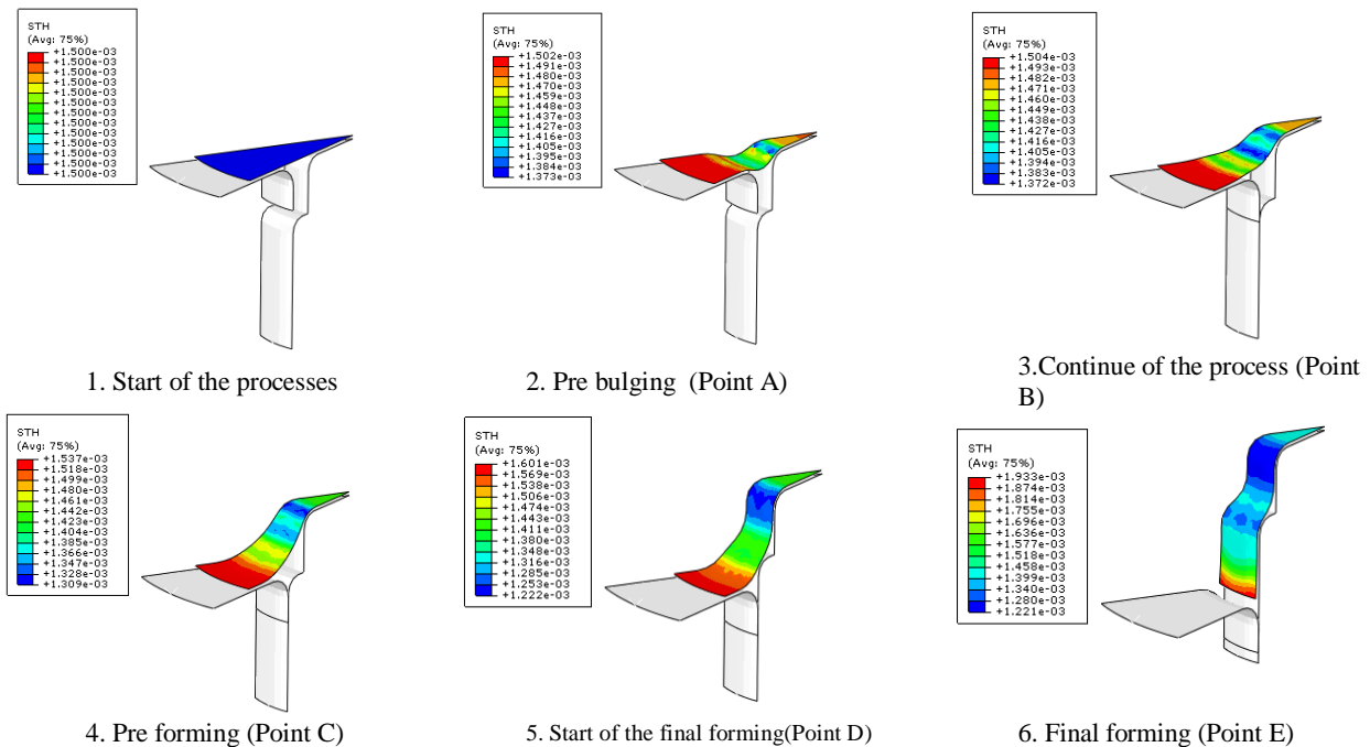
Fig 7. Simulation of the workpiece in hydroforming process in ABAQUS software
